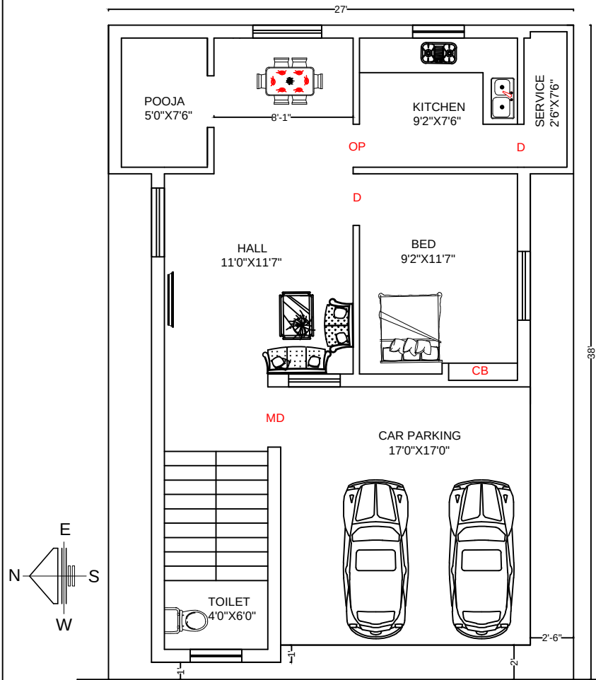
Road 24 feet GROUND FLOOR
