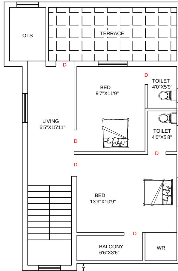
FIRST FLOOR Land Area - 1026 sq.ft Built Up Area - 1600 sq.ft
